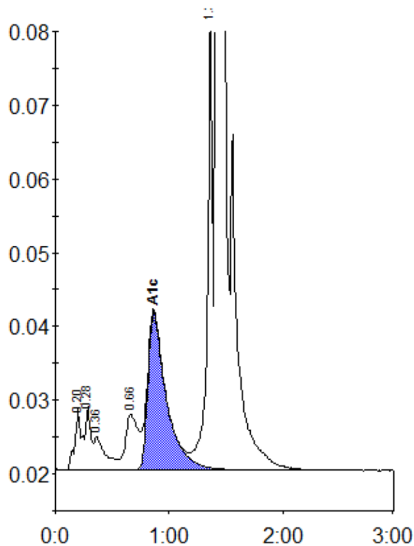
Peak table - ID: 10534374
